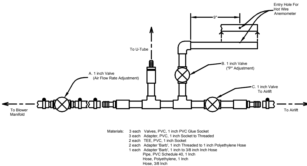
Figure 2. Air pressure flow regulator system for testing and adjusting air flow rates at various operating pressures.
