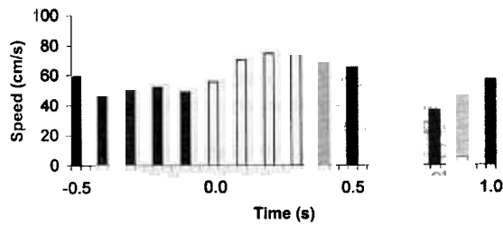
Fig. 6. Airspeed values for males exposed to binary blend (A) or the same binary blend with either 1% (B) or 10% (C) of Z11-16:Ac. White bars represent values occurring during the surge. Black bars correspond to values 0.5 s prior the surge and grey bars represent 0.4–1 s during it. Track angles prior the surge are significantly different than values in the time period 0.0–0.4 s after it ( P < 0.05 ).
