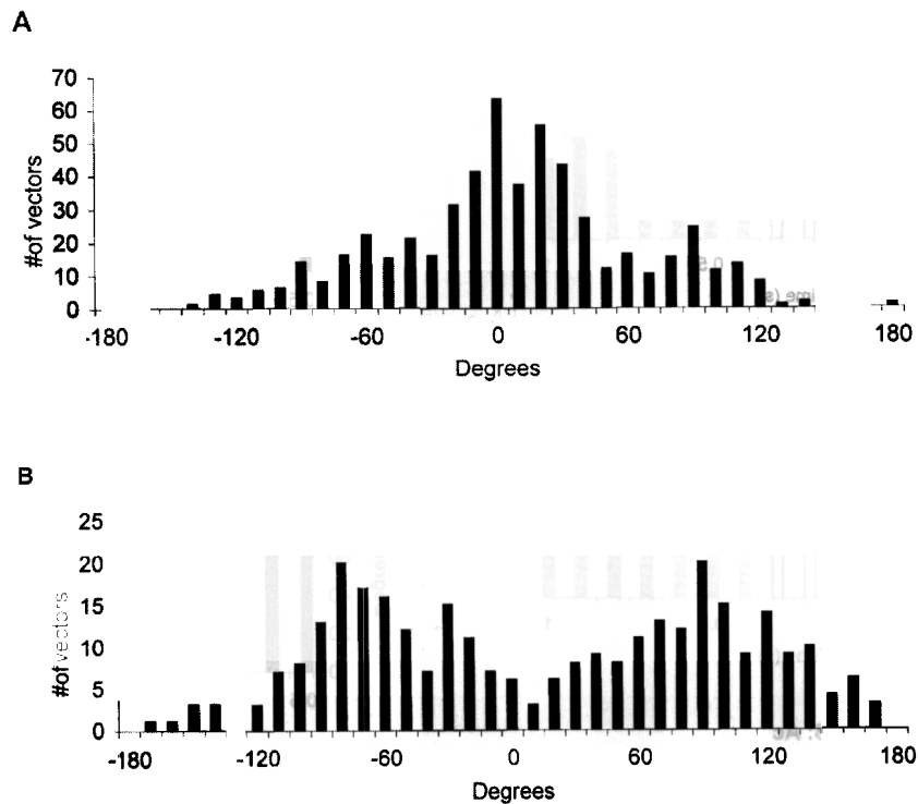
Fig. 3. Frequency distribution of track angle vectors for male flights during the 0.5 s before (A) and the 0.5–1 s after (B), flight into clean air. There is a unimodal distribution when males were flying in the plume ( n=10 ), and a bimodal distribution when the same males were casting in clear air ( n=10 ).
