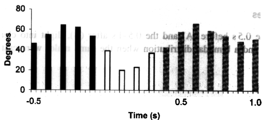
Fig. 4. Course angle values for males exposed to a single pulse of the binary blend (A) or to a pulse of the same binary blend with either 1% (B) or 10% (C) of Z11-16:Ac added. White bars represent values occurring during the upwind surge. Black bars correspond to values 0.5 s prior the surge and grey bars represent 0.4–1 s after it. Track angles prior the surge are significantly different than values in the time period 0.0–0.4 s during it ( P < 0.05 ).
