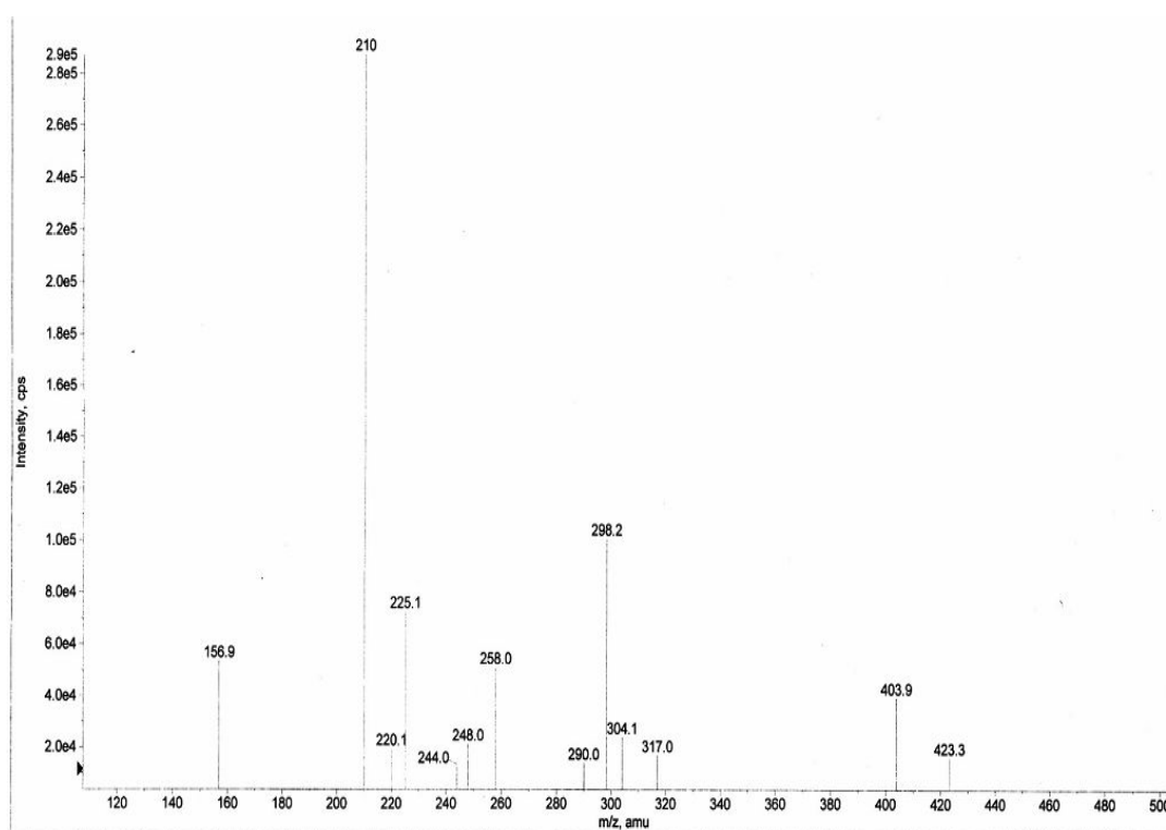
Fig. 2. Mass Spectra of 2, 4-Diacetylphloroglucinol produced by Pseudomonas fluorescens strain p.f.05.
